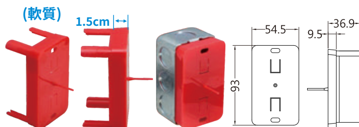
BA144 BOX修飾蓋
